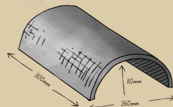
HALF ROUND RIDGE
