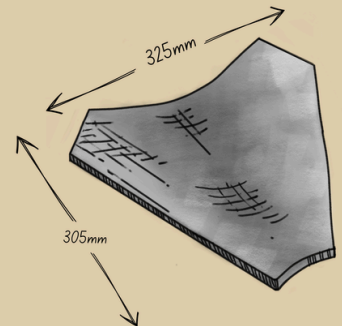
HALF ROUND RIDGE
